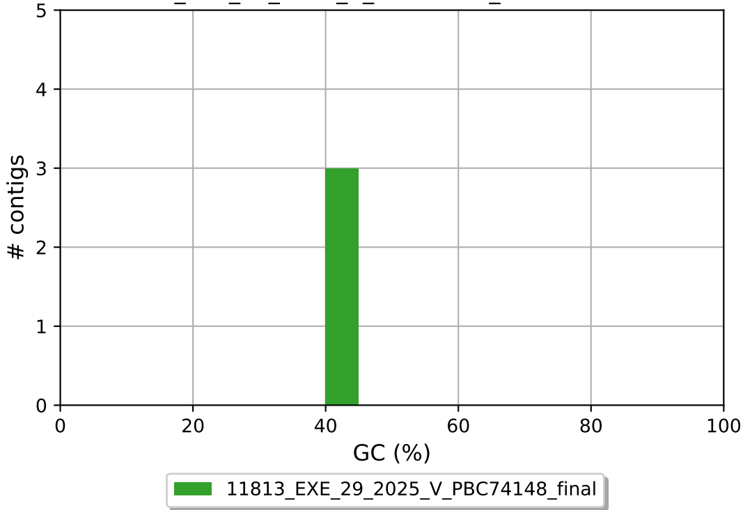
11813_EXE_29_2025_V_PBC74148_final GC content
