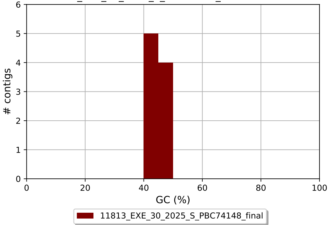
11813_EXE_30_2025_S_PBC74148_final GC content
