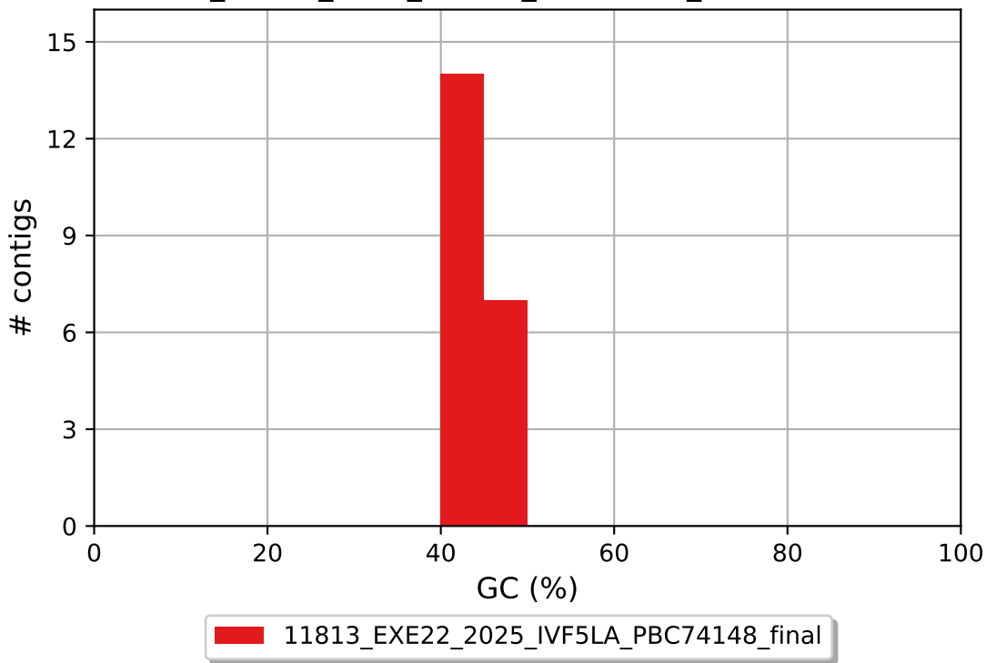
11813_EXE22_2025_IVF5LA_PBC74148_final GC content
