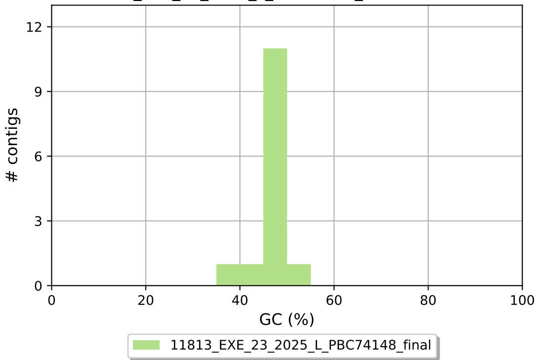
11813_EXE_23_2025_L_PBC74148_final GC content
