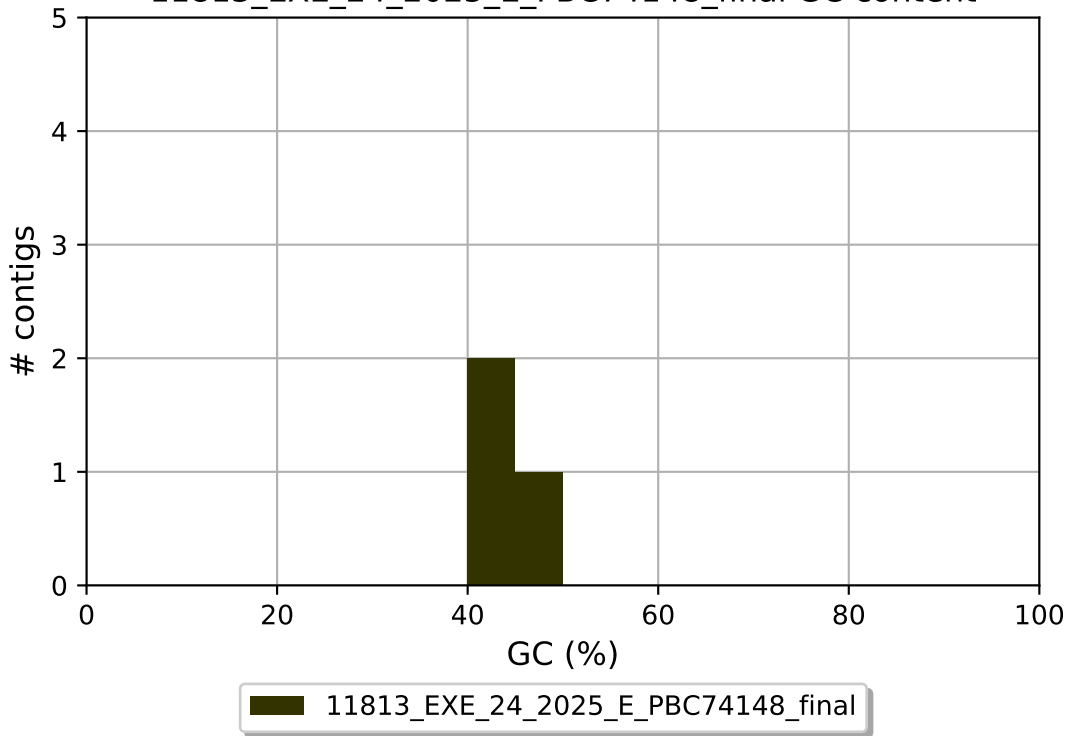
11813_EXE_24_2025_E_PBC74148_final GC content
