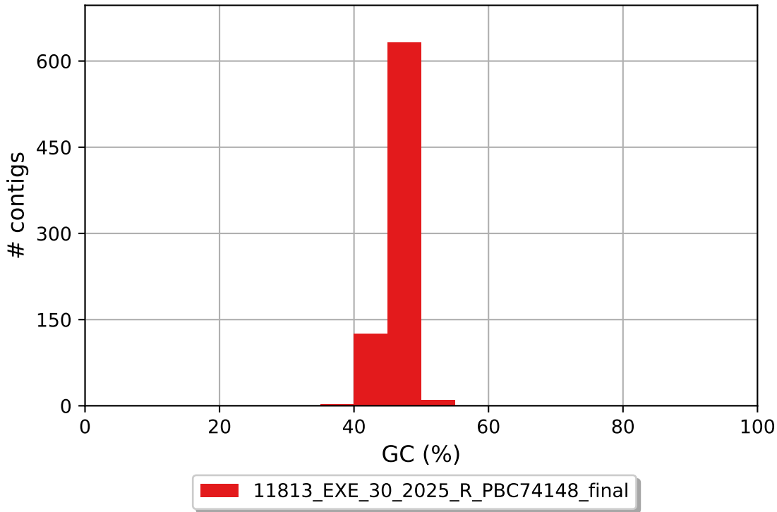
11813_EXE_30_2025_R_PBC74148_final GC content
