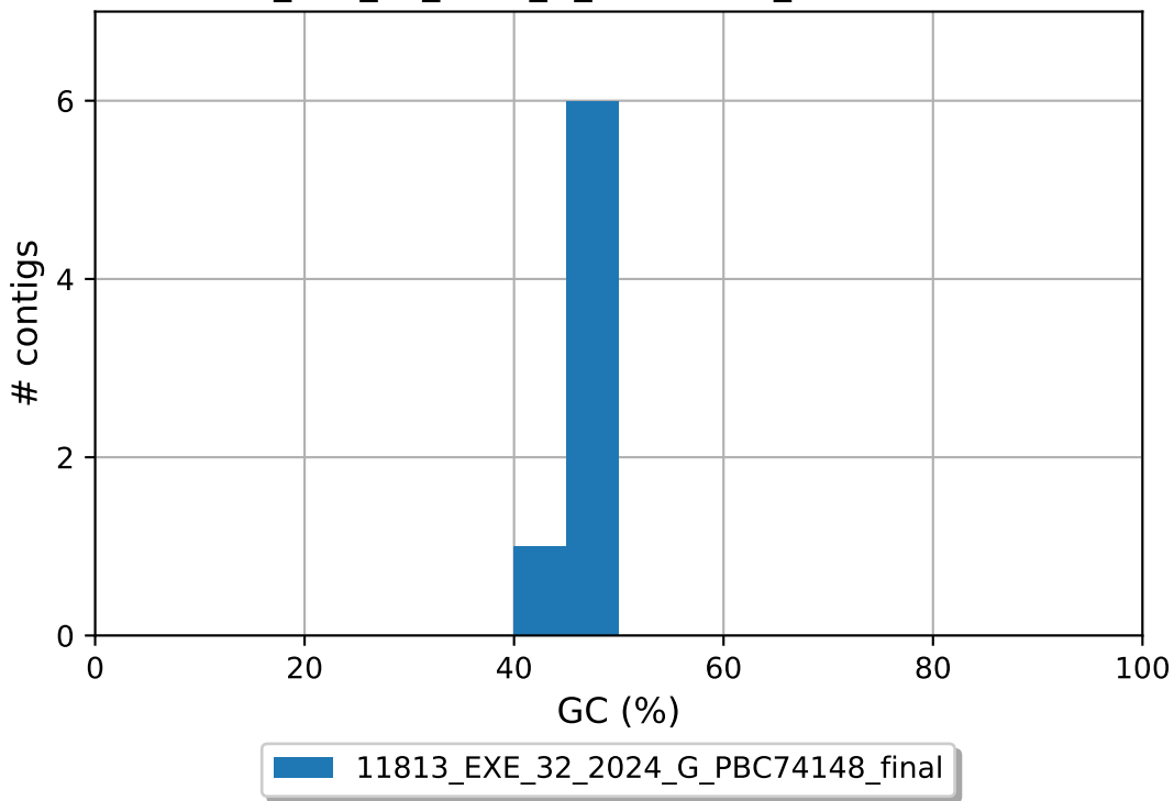
11813_EXE_32_2024_G_PBC74148_final GC content
