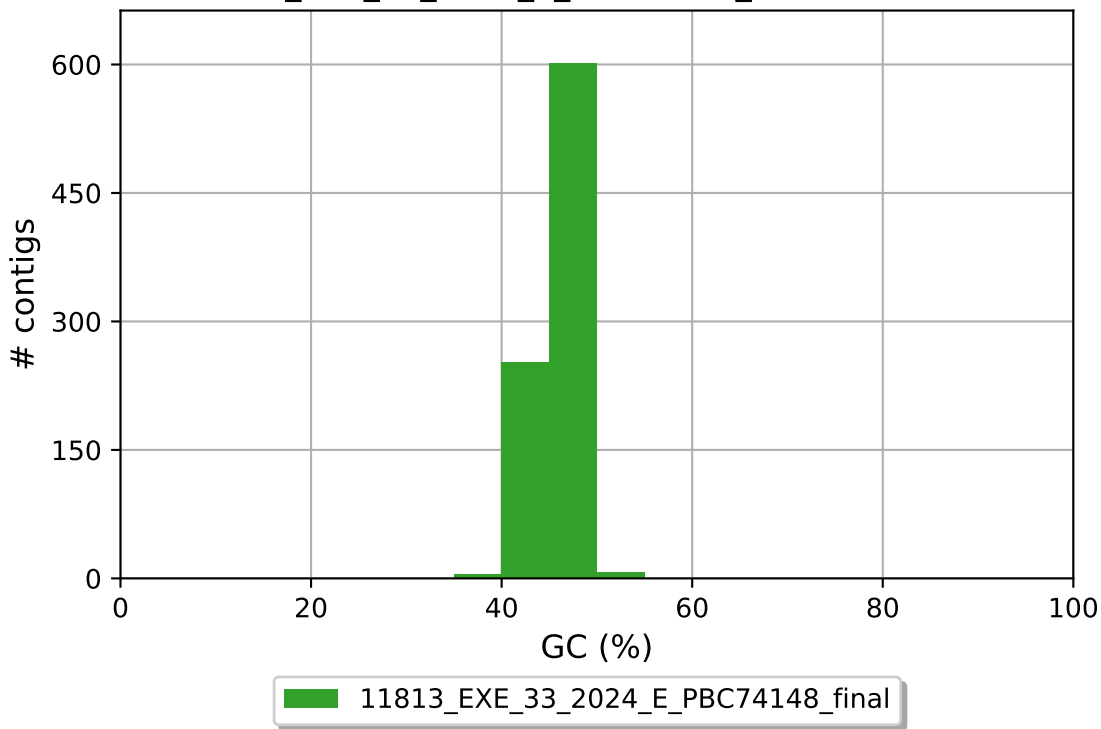
11813_EXE_33_2024_E_PBC74148_final GC content
