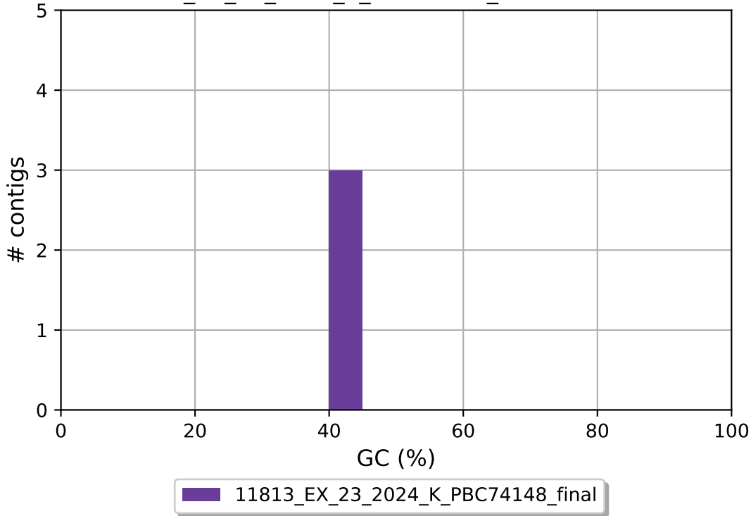
11813_EX_23_2024_K_PBC74148_final GC content
