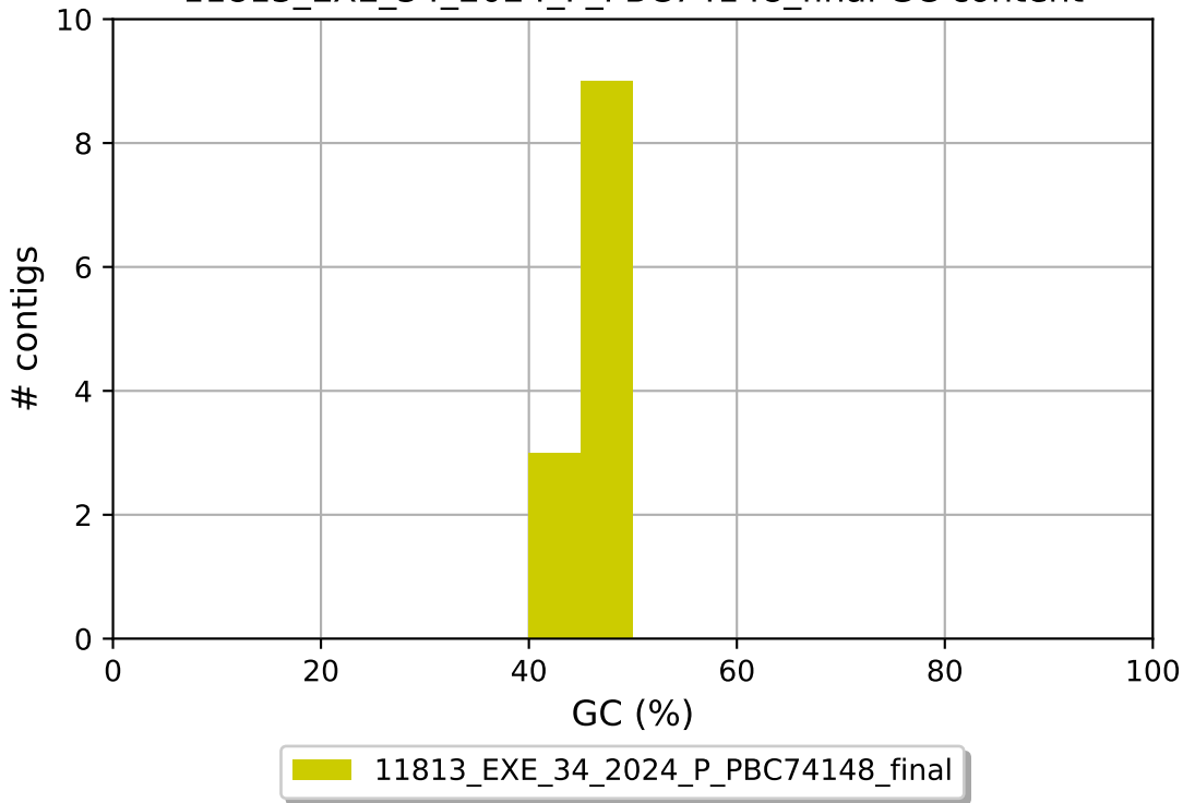
11813_EXE_34_2024_P_PBC74148_final GC content
