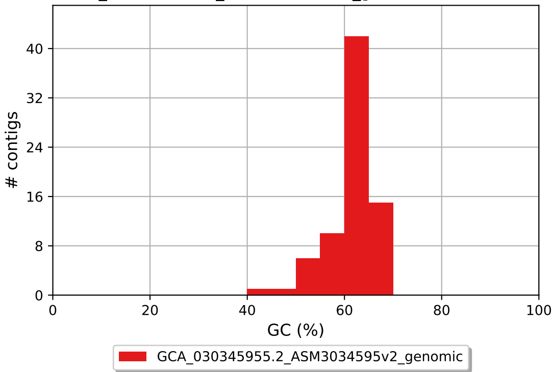
GCA_030345955.2_ASM3034595v2_genomic GC content
