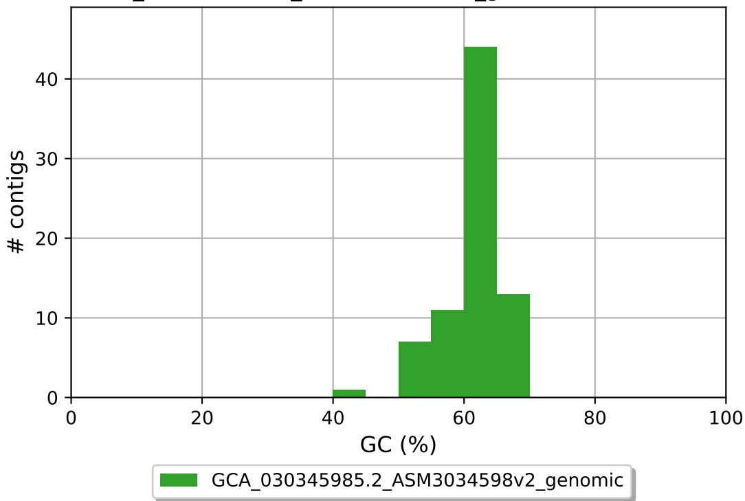
GCA_030345985.2_ASM3034598v2_genomic GC content
