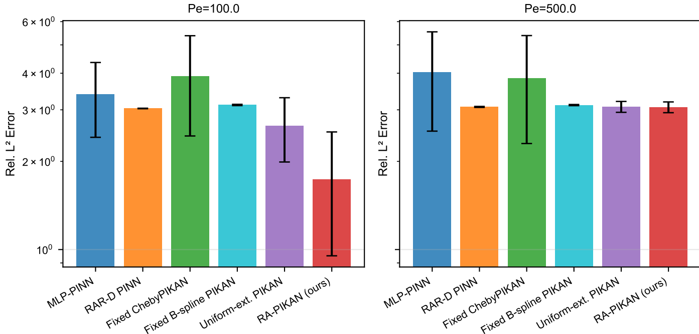
Adv-Diff: Final L^2 Error by Method
