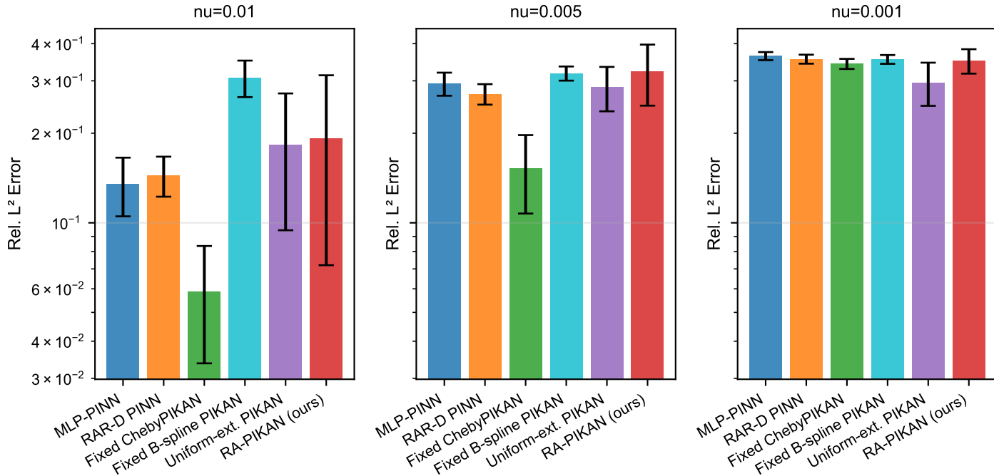
Burgers: Final L^2 Error by Method
