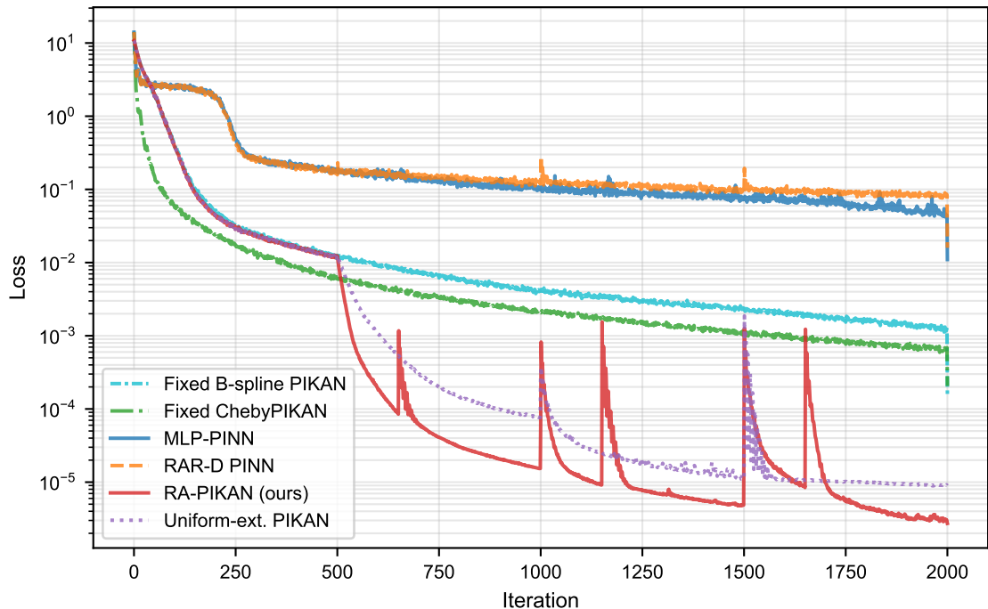
Convergence: allen_cahn (eps0.05_seed42)
