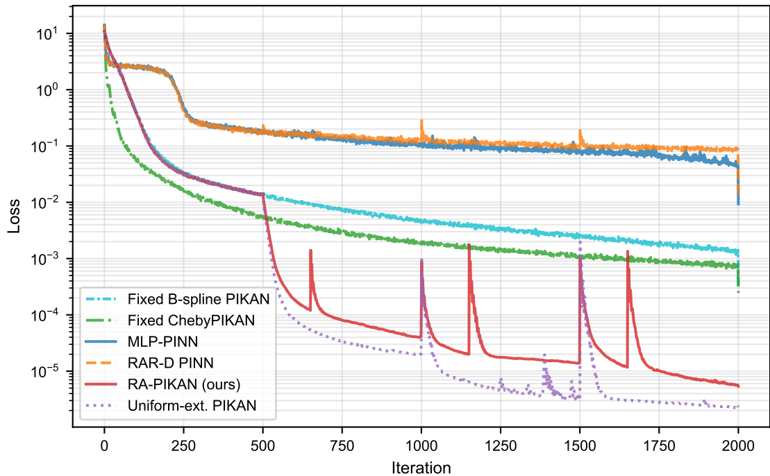
Convergence: allen_cahn (eps0.1_seed42)
