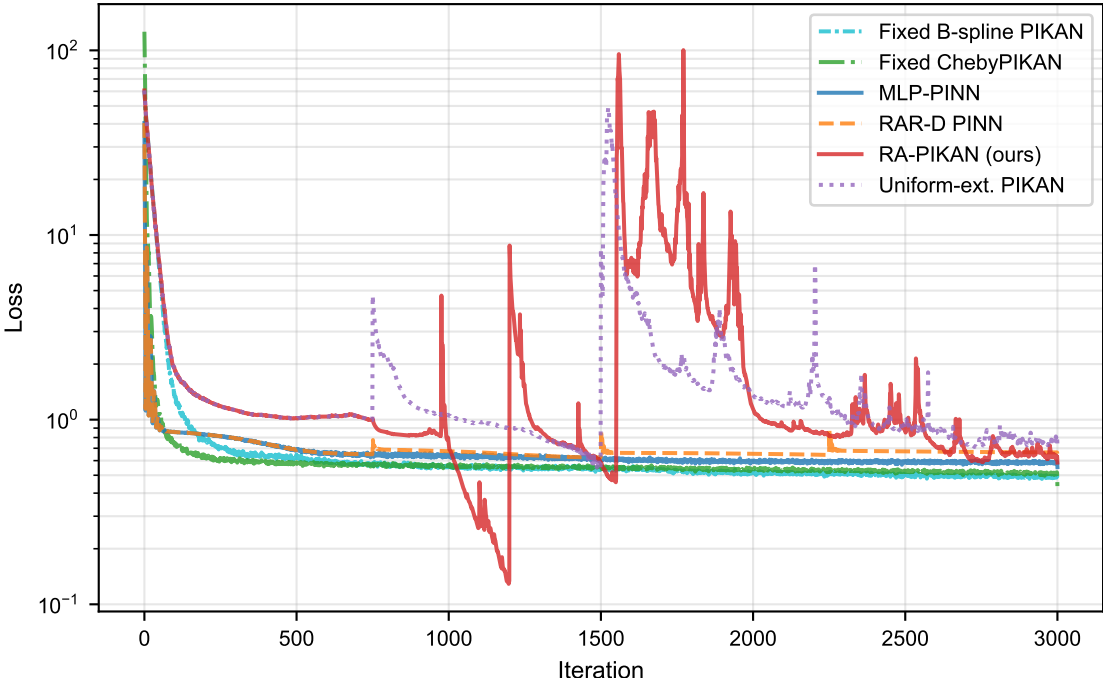
Convergence: adv diff (Pe100.0 seed42)
