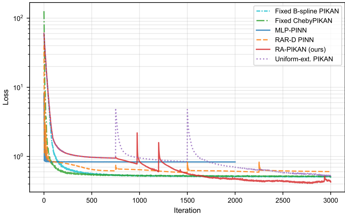
Convergence: adv_diff (Pe500.0_seed42)
