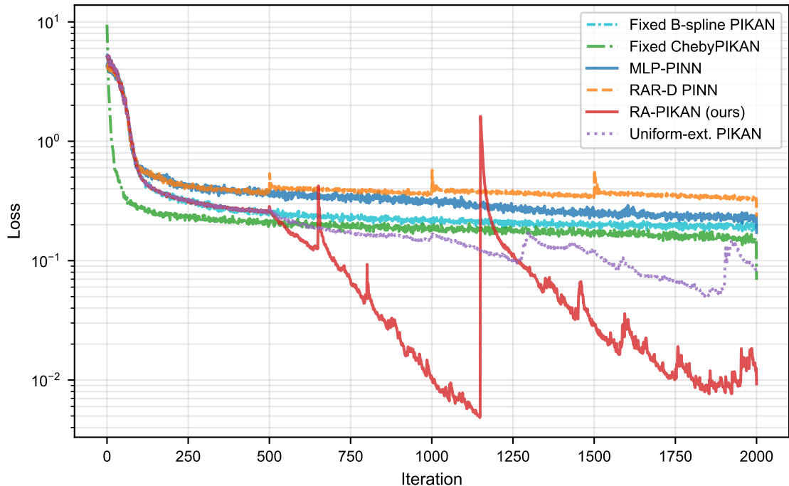
Convergence: burgers (nu0.005_seed42)
