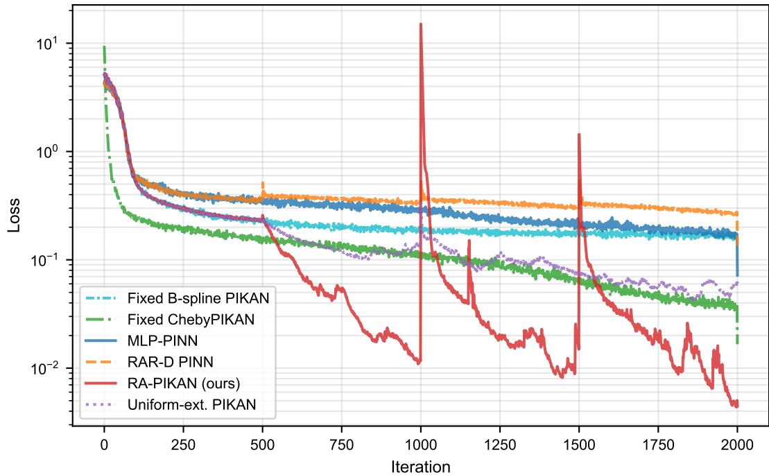
Convergence: burgers (nu0.01_seed42)
