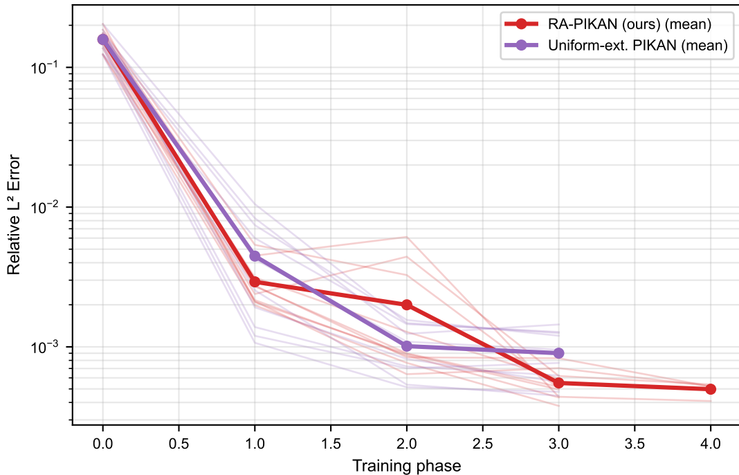
L^2 error per phase: Allen-Cahn (eps0.05), 10 seeds
