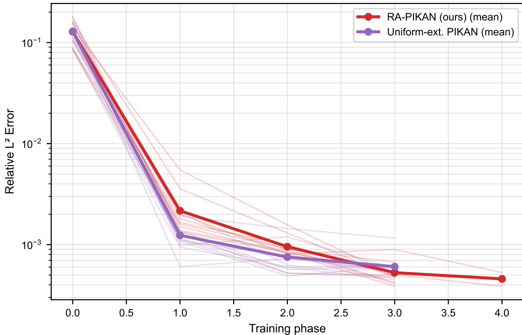
L^2 error per phase: Allen-Cahn (eps0.1), 10 seeds
