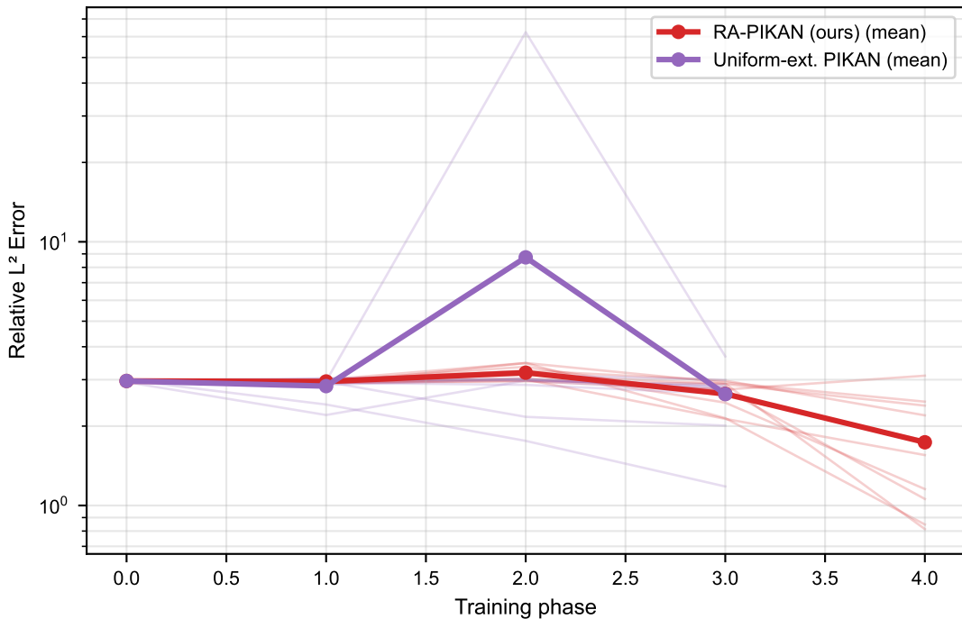
L^2 error per phase: Adv-Diff (Pe100.0), 10 seeds
