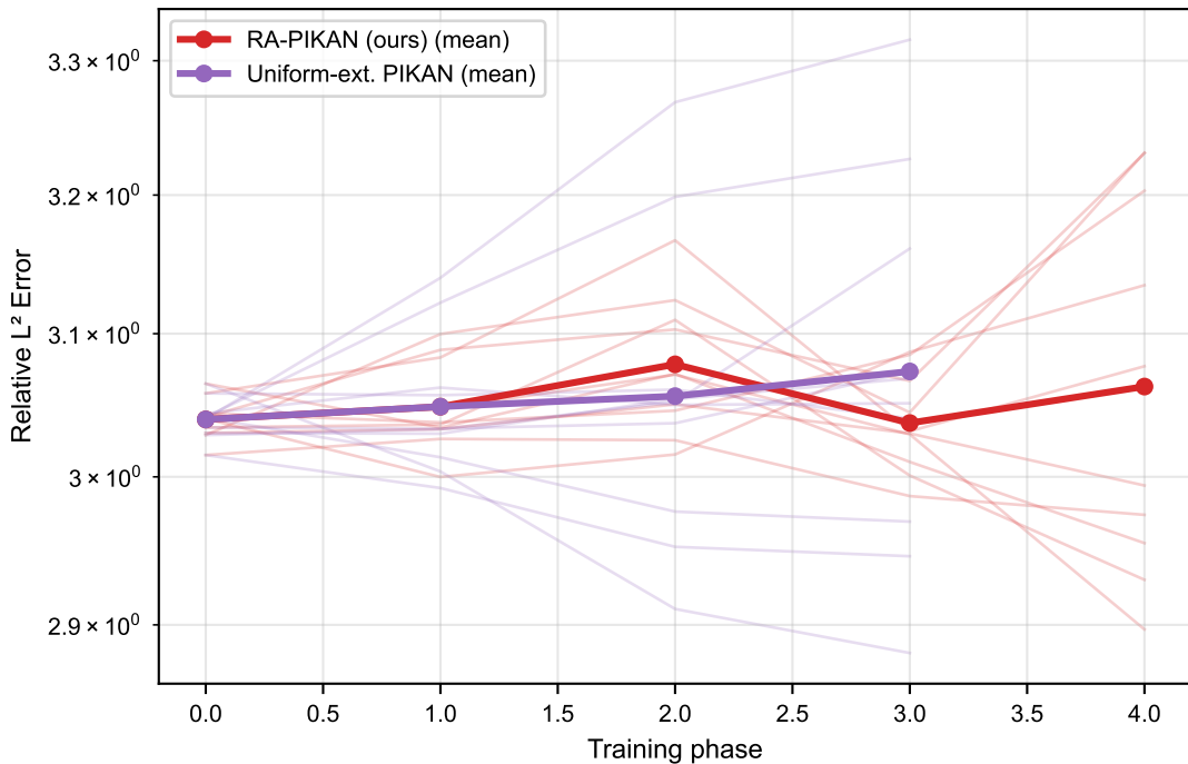
L^2 error per phase: Adv-Diff (Pe500.0), 10 seeds
