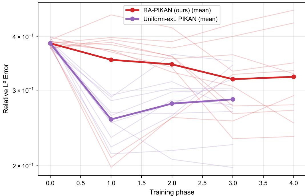
L 2 error per phase: Burgers (nu0.005), 10 seeds
