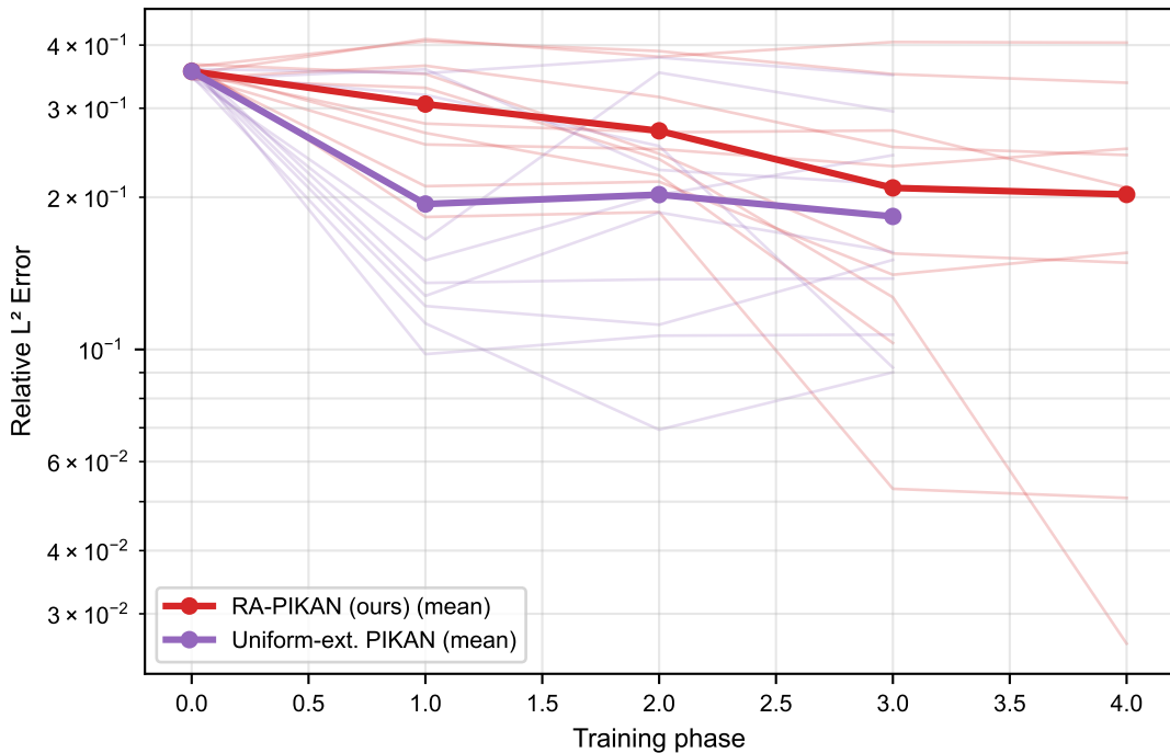
L^2 error per phase: Burgers (nu0.01), 10 seeds
