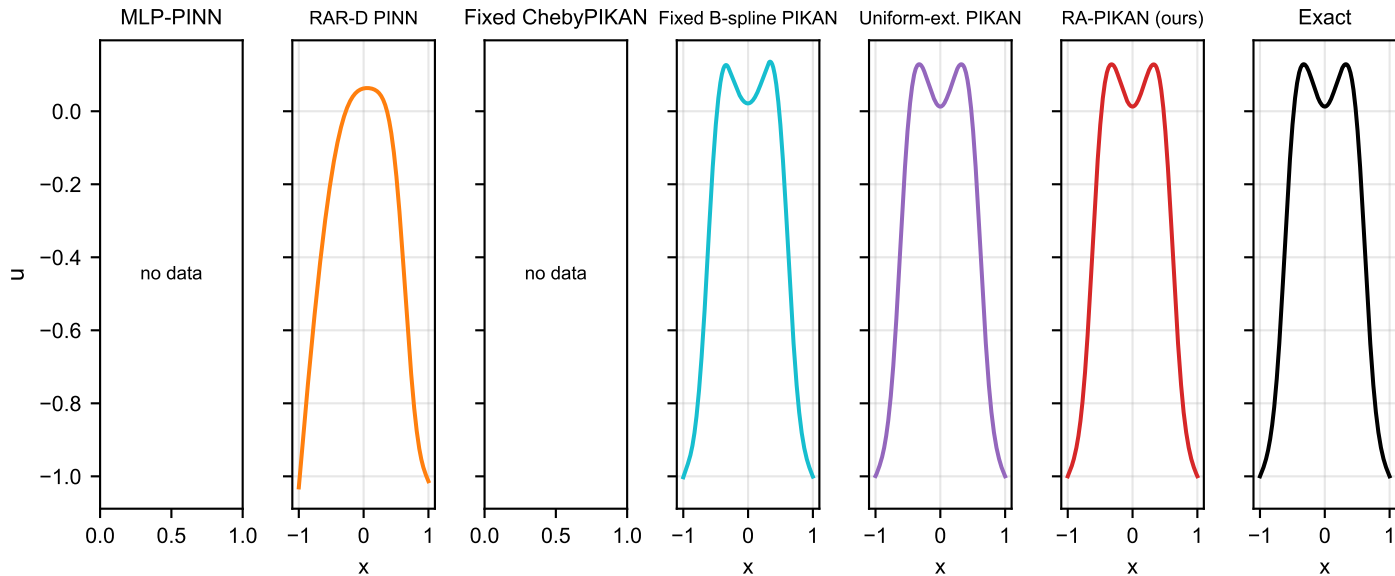
Solution profiles: allen_cahn (eps=0.05, t=final)
