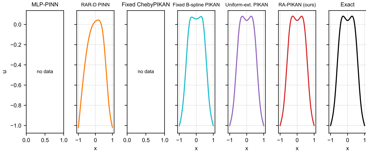
Solution profiles: allen_cahn (eps=0.1, t=final)
