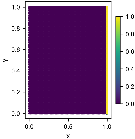
Exact
