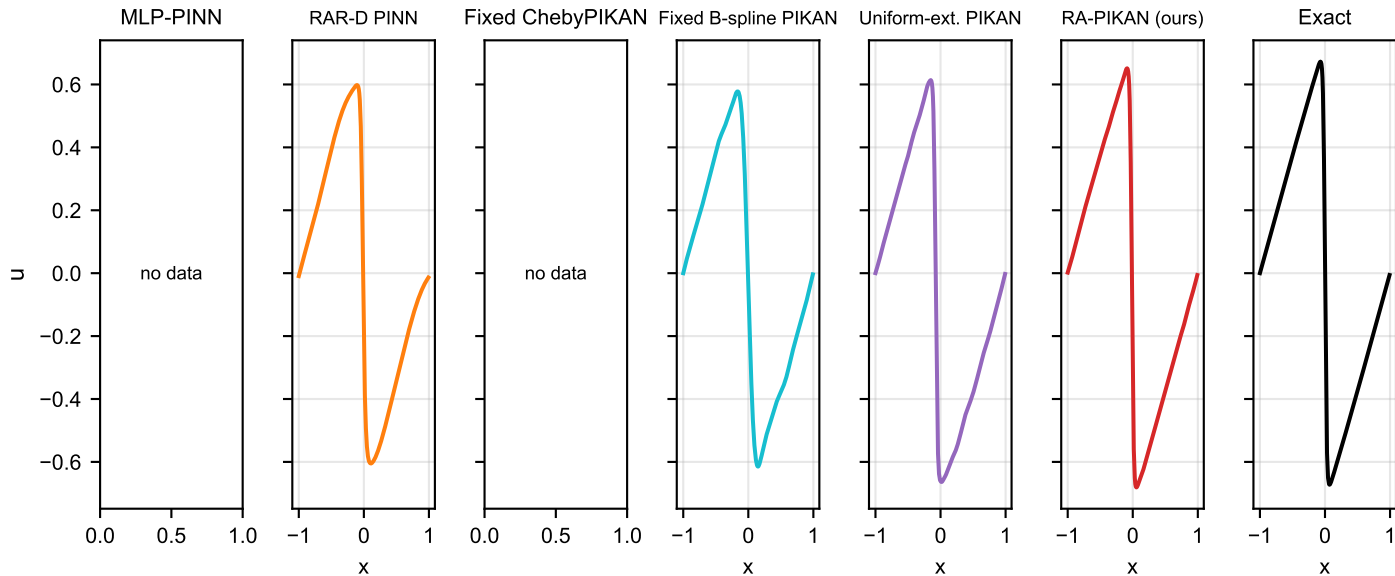
Solution profiles: burgers (nu=0.01, t=final)
