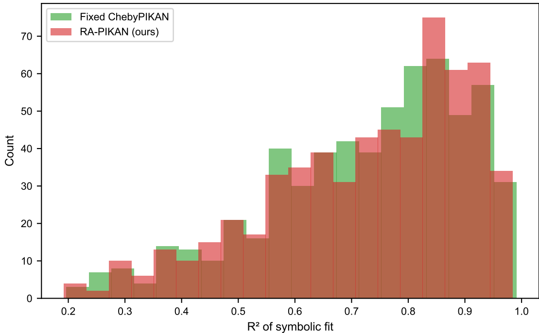
Symbolic Extraction: R^2 Distribution (Duffing)
