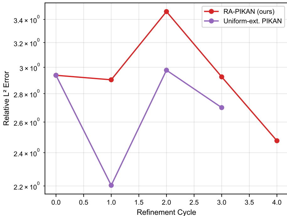
L2 Error vs Cycle: adv_diff (Pe100.0_seed42)
