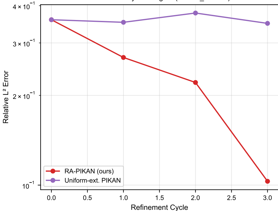
L2 Error vs Cycle: burgers (nu0.01_seed42)
