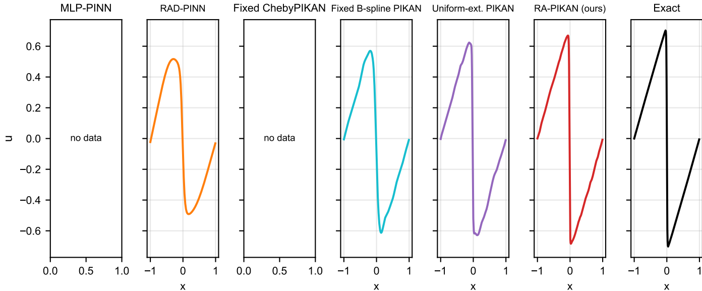
Solution profiles: burgers (nu=0.005, t=final)
