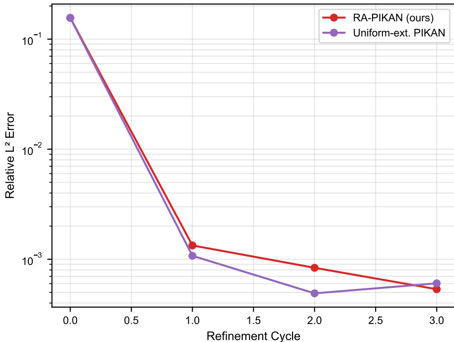
L2 Error vs Cycle: allen_cahn (eps0.1_seed42)
