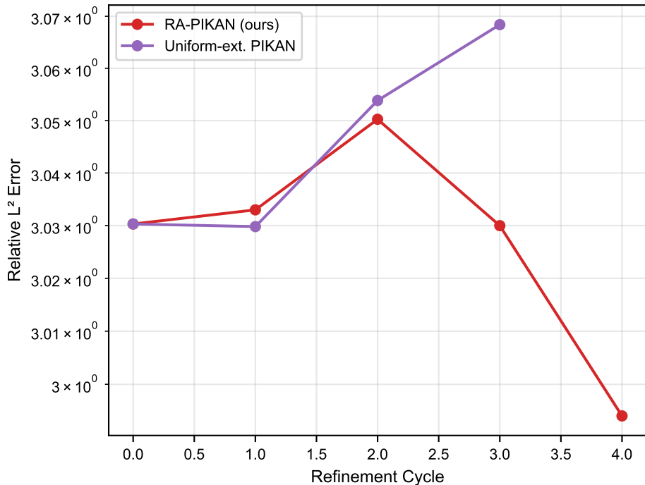
L2 Error vs Cycle: adv_diff (Pe500.0_seed42)
