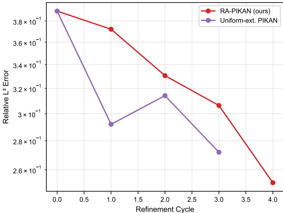
L2 Error vs Cycle: burgers (nu0.005_seed42)
