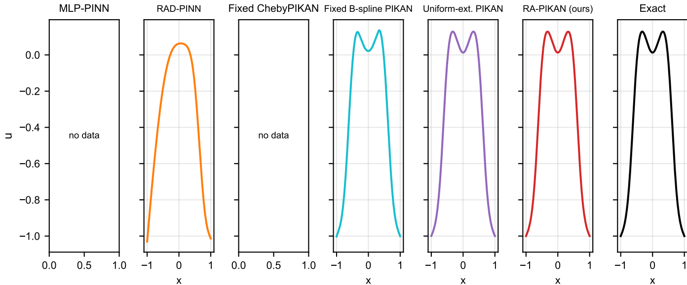
Solution profiles: allen_cahn (eps=0.05, t=final)
