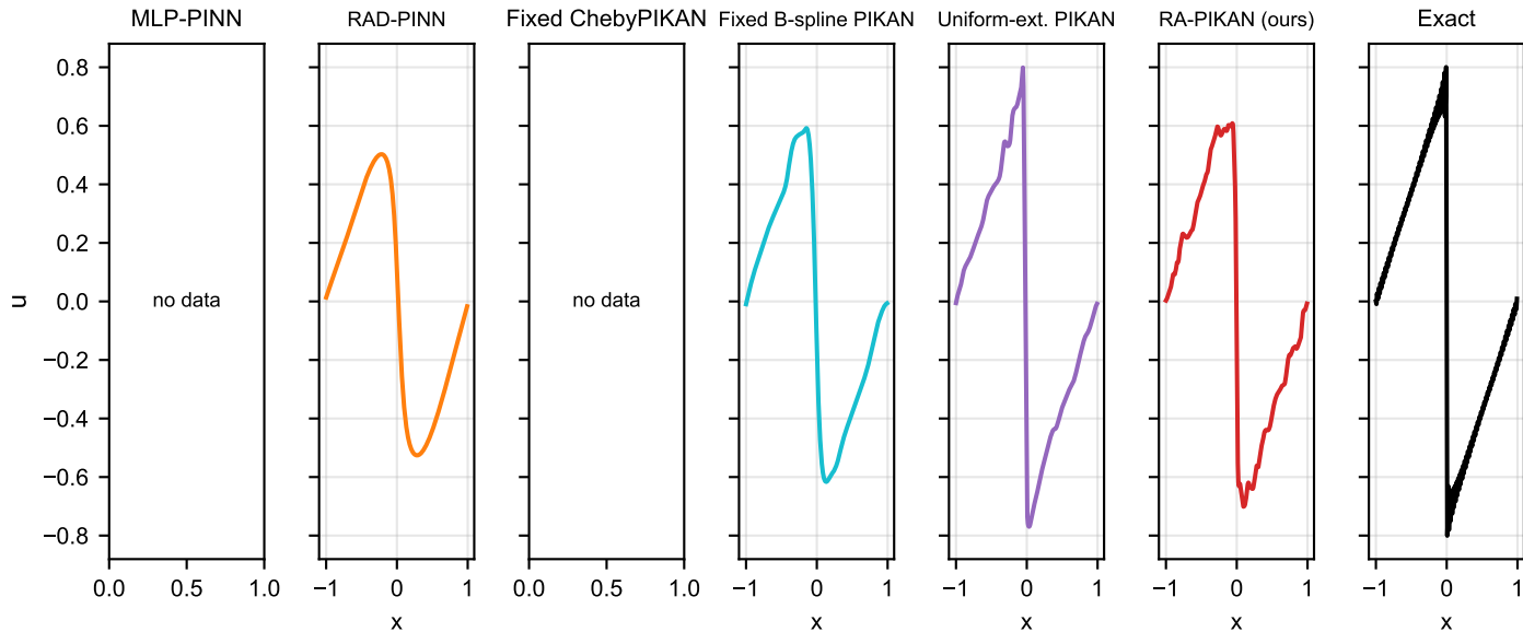
Solution profiles: burgers (nu=0.001, t=final)
