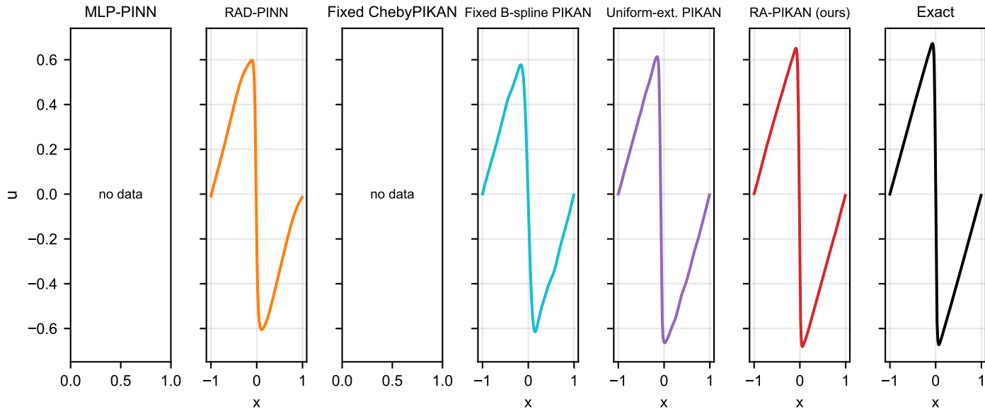
Solution profiles: burgers (nu=0.01, t=final)
