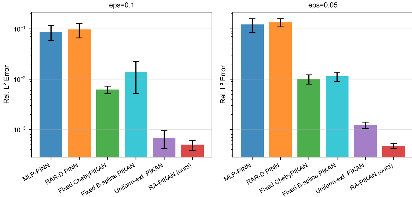
Allen-Cahn: Final L^2 Error by Method
