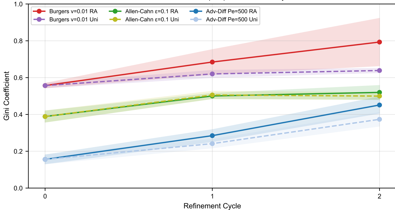
Residual Concentration (Gini) vs Refinement Cycle
