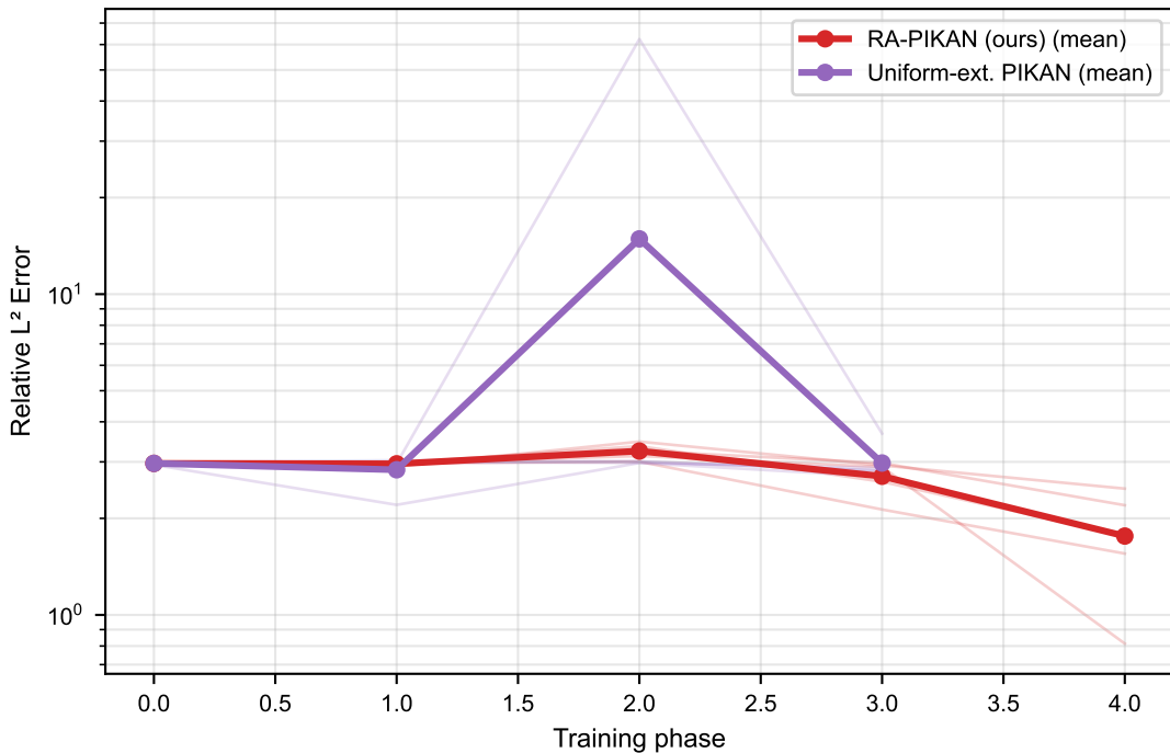
L^2 error per phase: Adv-Diff (Pe100.0), 5 seeds
