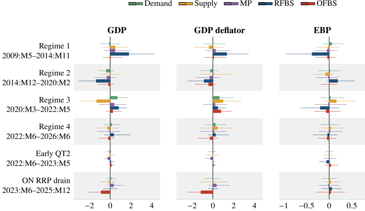
Figure 7: Historical decomposition by volatility regime.
