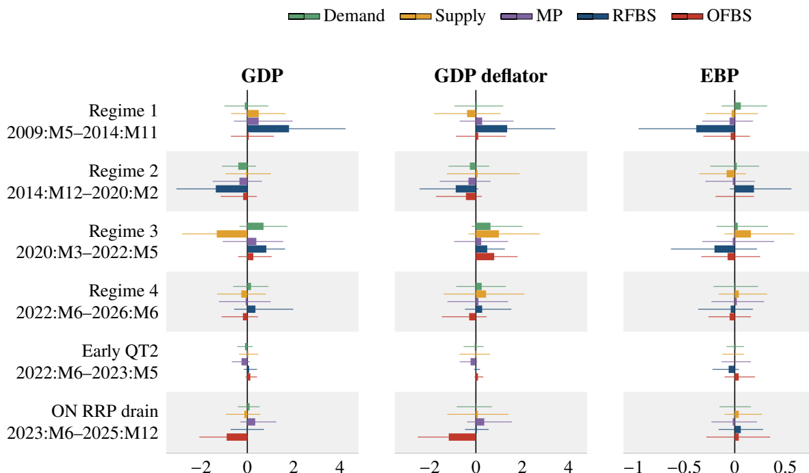
Figure 8: Historical decomposition by volatility regime.
