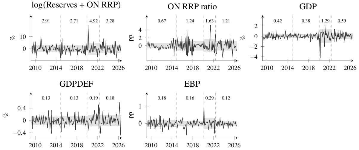
Figure D.1: Reduced-form residuals under a single variance regime, the remaining five equations. Note. The equations Figure 5 leaves out, on the same estimation and with the same bands and subsample standard deviations. Units are percent for the log levels and percentage points for the ratio and the premium.
