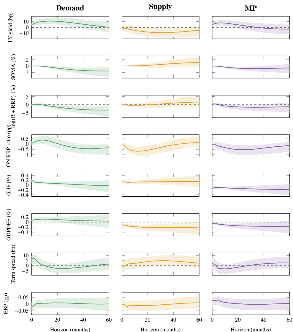
Figure F.1: Impulse responses to the demand, supply, and MP shocks.
