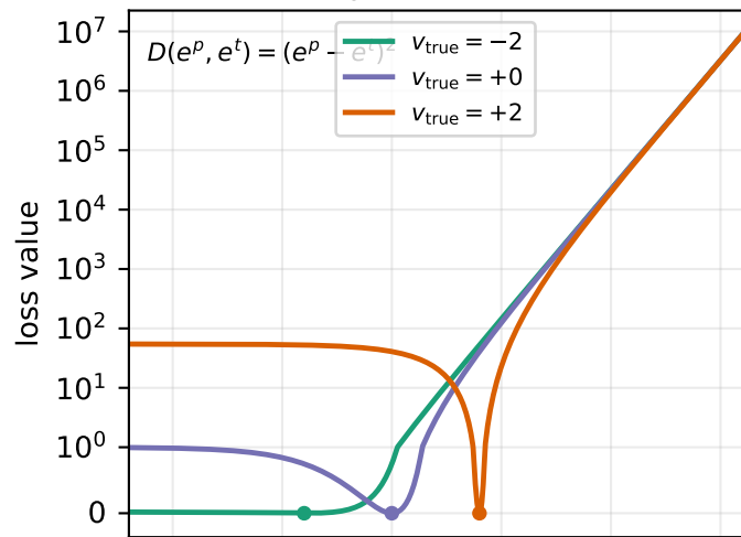
Squared error
