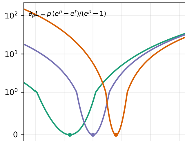
Spence (ours)
