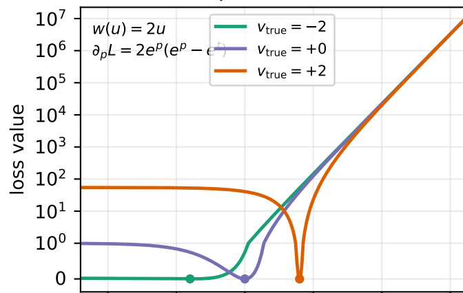
Squared error
