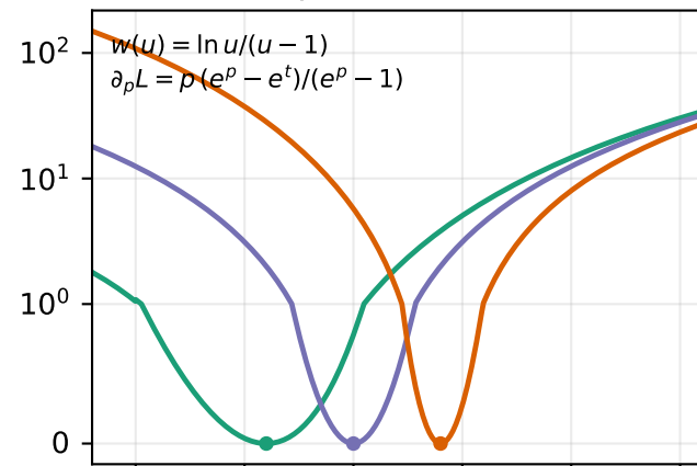
Spence (ours)
