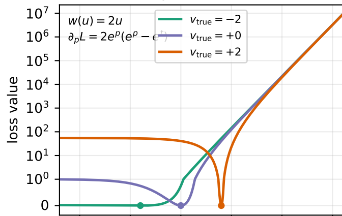
Squared error
