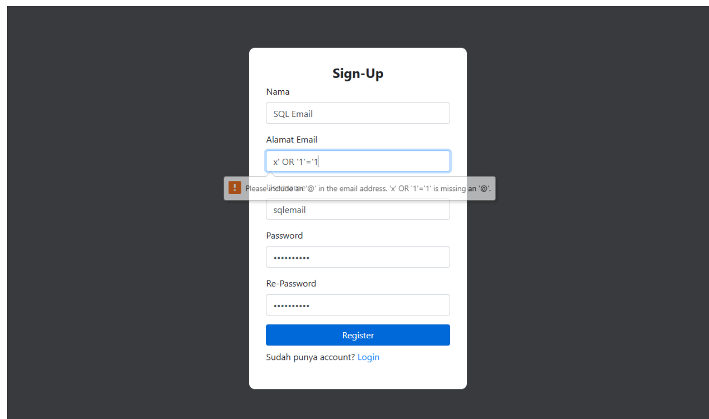
test_register_email_sql_injection_FAIL.png
